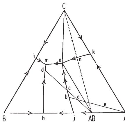
FIG. XVII.—Ternary system containing a binary compound unstable at its melting point.
