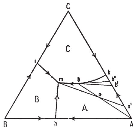
FIG. XV.—Course of crystallization in a simple ternary system O. Andersen, Am. J. Sci. , 4th Ser., 39, 427 (1915).
